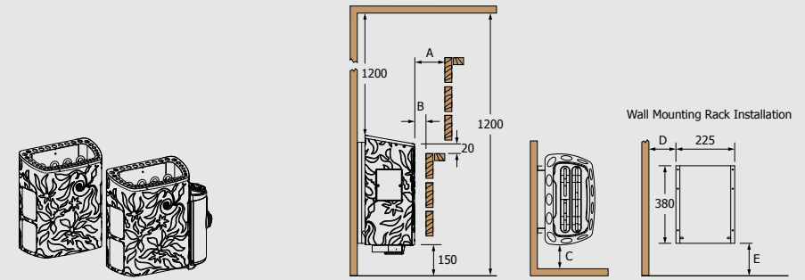
Minidragon
